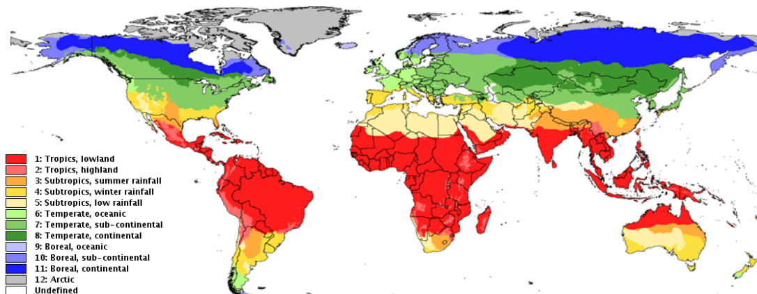
Figure 3-2 Thermal climates
