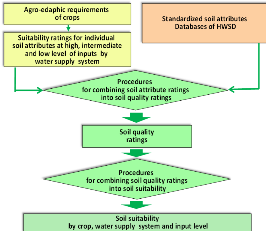
Figure 6-3 Soil suitability rating procedures
